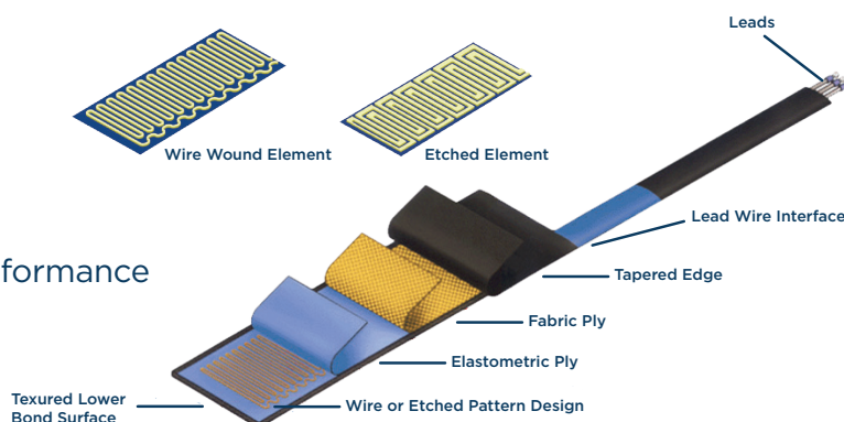
Engine Inlet De-icers
